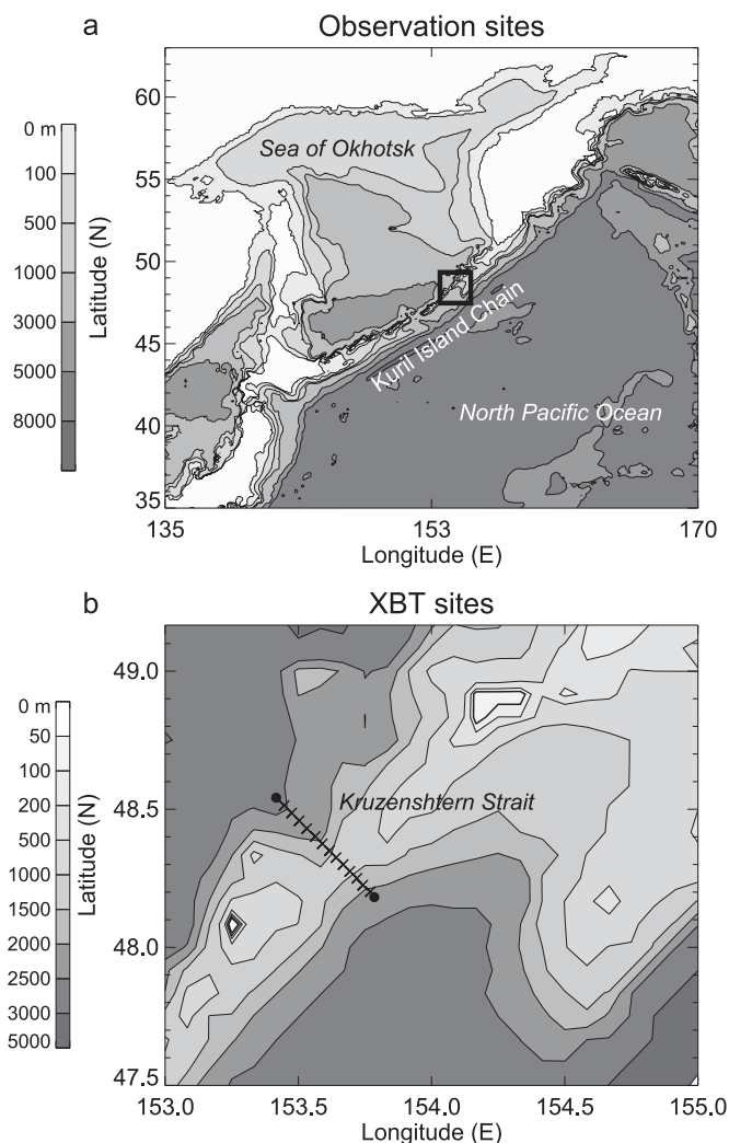
Fig. 1. Observation sites. (a) Location of the Kruzenshtern Strait and the Kuril Island Chain. (b) Observation sites and topography. Crosses and solid circles indicate the sites of XBT and CTD measurements, respectively.
