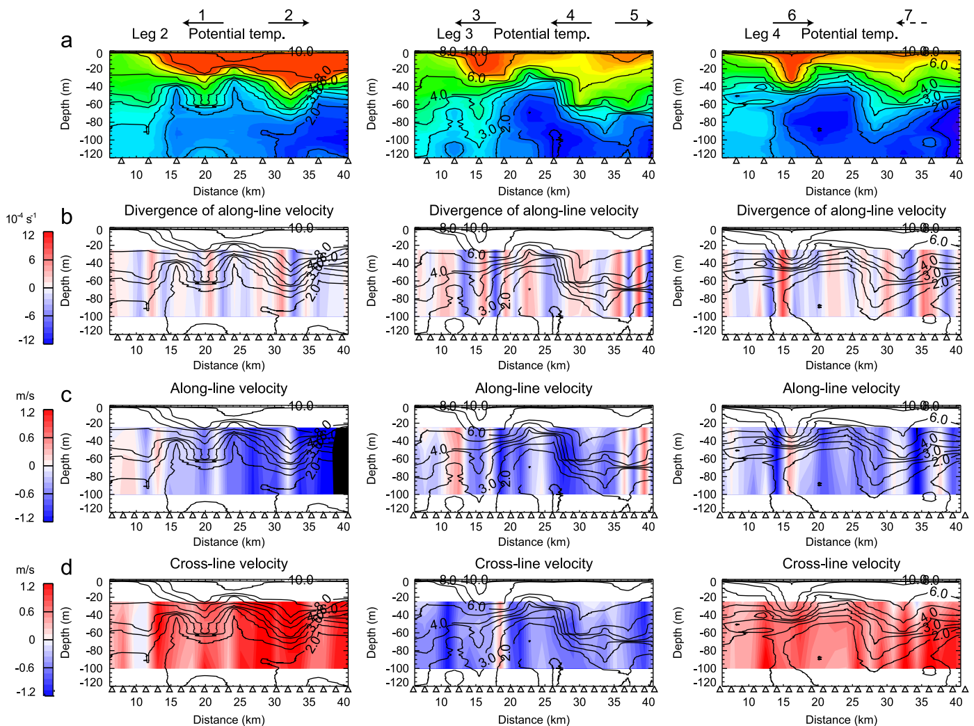
Fig. 4. Vertical sections of (a) potential temperature, (b) divergence of along-line velocity, (c) along-line velocity, and (d) cross-line velocity observed in legs 2–4 from left to right. Triangles below each panel indicate the locations of measurements.
