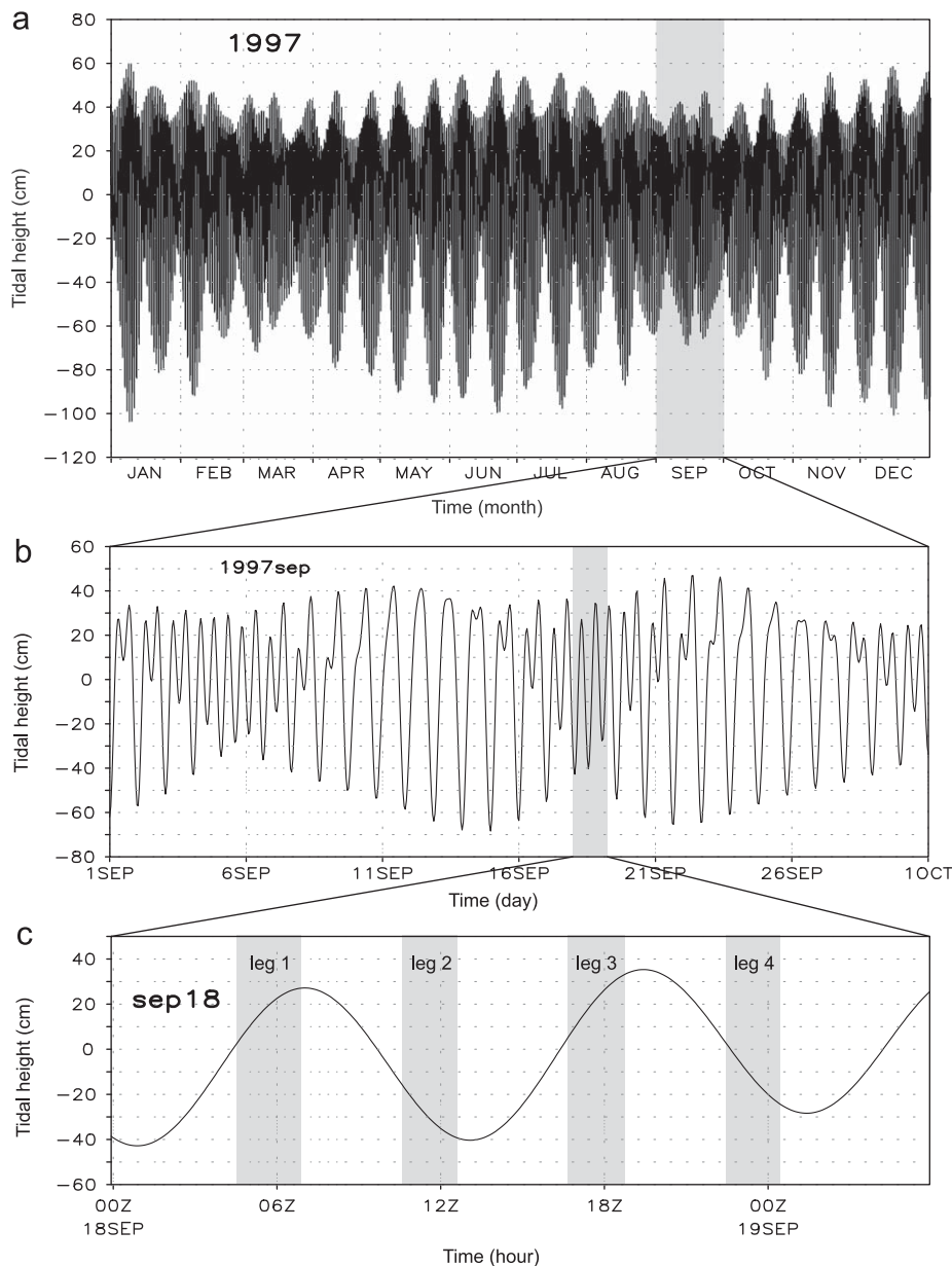
Fig. 2. The time duration of the observation and tidal height during (a) 1997, (b) September 1997, and on (c) 18–19 September 1997. Shaded areas in the bottom panel show the observation duration. Tidal height is calculated based on Matsumoto et al. (2000) at the location of the sill on the observation line.
