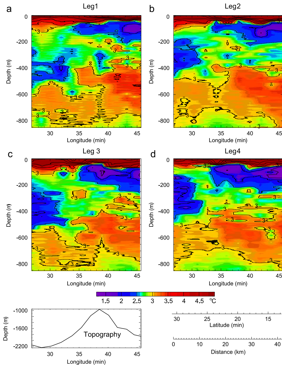
Fig. 3. Vertical sections of potential temperature and the bottom topography along the observation line. Contour intervals are 0.5^{\circ}\text{C} for \leq 3^{\circ}\text{C} and 1^{\circ}\text{C} for >3^{\circ}\text{C} . The North Pacific Ocean (the Sea of Okhotsk) is on the right (left) hand side.
