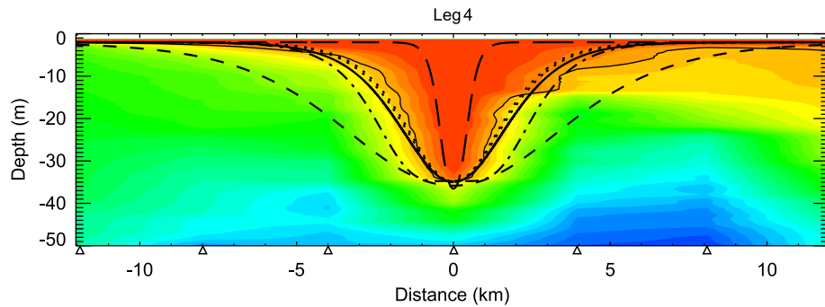
Fig. 5. Comparison of the observed isotherm depression 6 in Fig. 4 and solutions of Miyata soliton (thick solid line), KdV and eKdV solitons (dotted line), and JKKD soliton (short dashed line), using parameter values selected so as to fit the former three soliton solutions to the shape of the isotherms ( h_1 = 240 m where h_1 corresponds to the upper layer thickness in a two-layer fluid system). The KdV and eKdV soliton solutions are indistinguishable in this figure. Also shown are a JKKD soliton (dash dot) which is fitted to the isotherm shape ( h_1 = 60 m) and a JKKD soliton (long dash) which is obtained by assuming that the pycnocline experienced by the wave lies close to the sea surface ( h_1 = 15 m).
