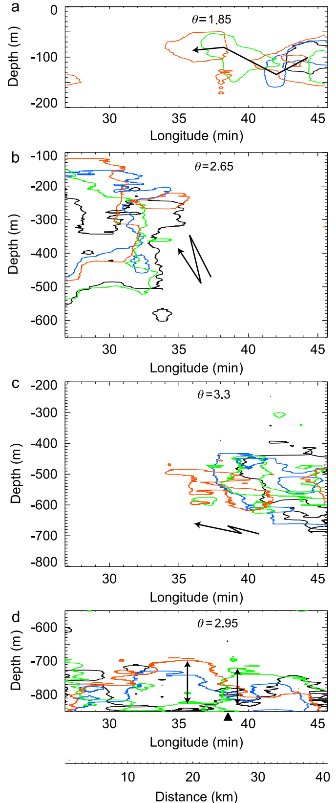
Fig. 6. Isotherms selected to show the movements of water masses. Black, blue, green and red contours represent isotherms observed in legs 1–4, respectively. The solid triangle below the panel (d) indicates the location of the sill top.
